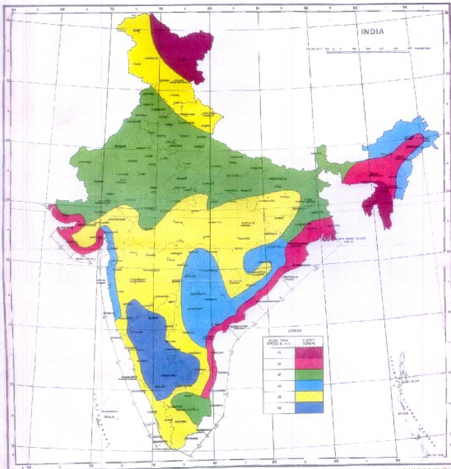
FIG. 1. BARD WIND SPEED (m/s) (BASED ON 50-YEAR RETURN PERIOD)
